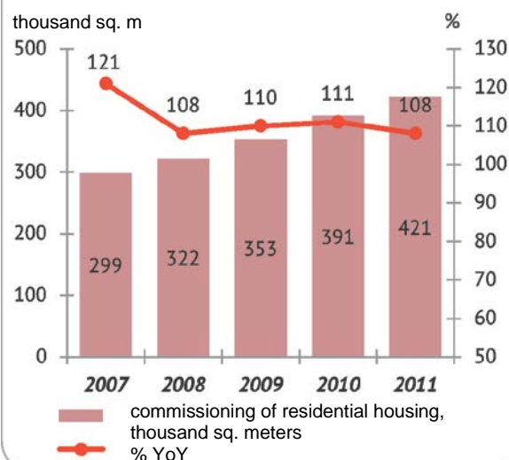
Housing construction dynamics
