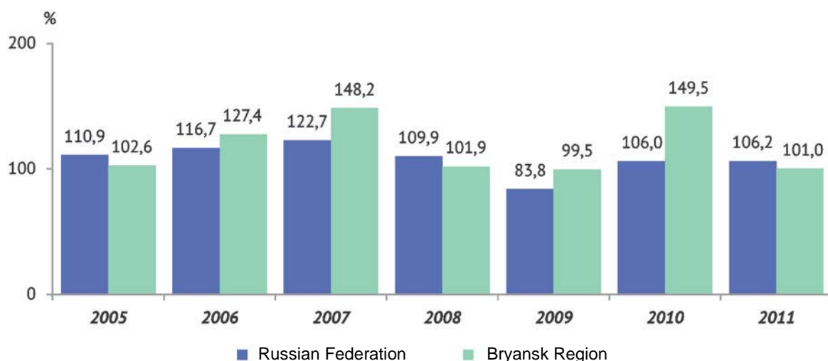
Capital investments physical volume dynamics
